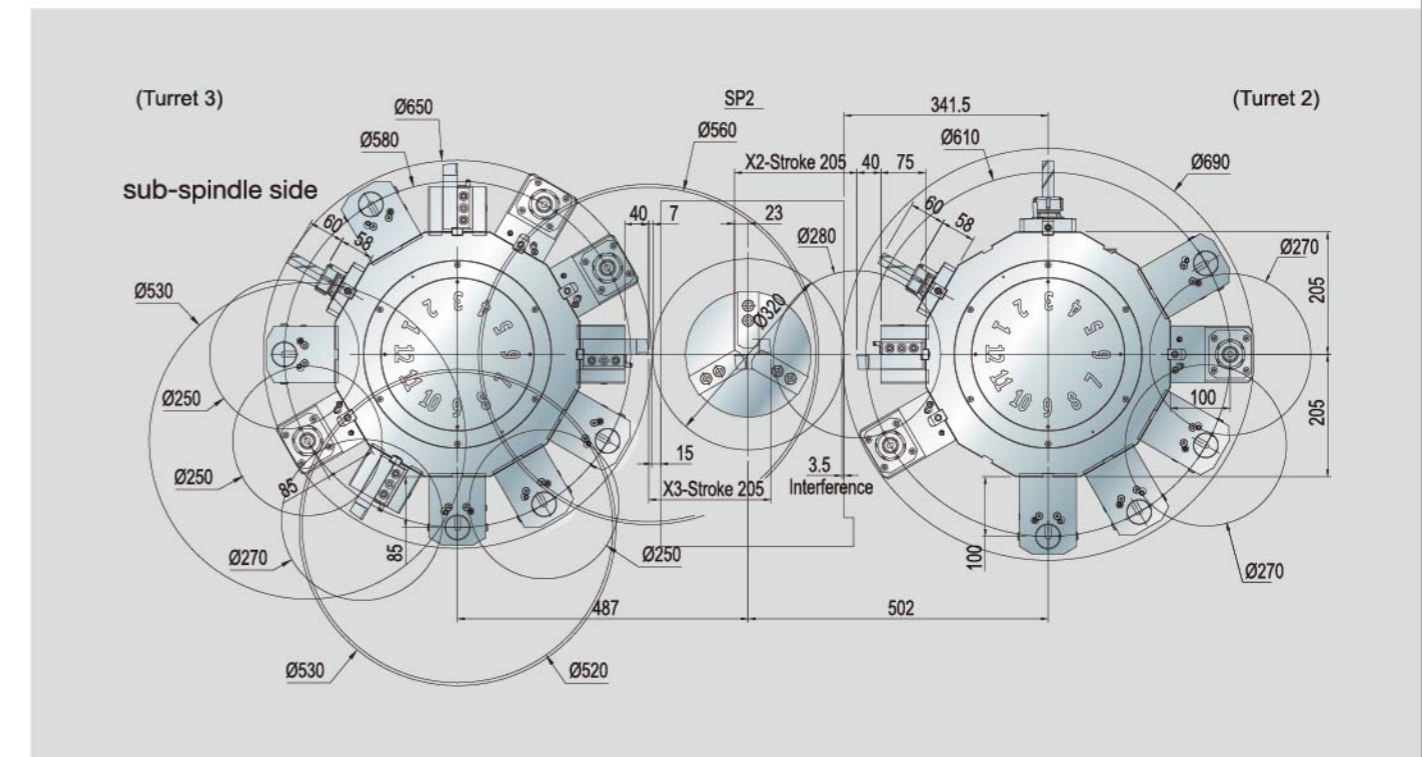
(Turret 3) ID tool holder with center height 85 mm/(Turret 2) ID tool holder with center height 100 mm
